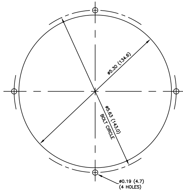
4-1/2 in. DIAL PANEL CUT-OUT
