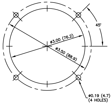
2-1/2 in. DIAL PANEL CUT-OUT
